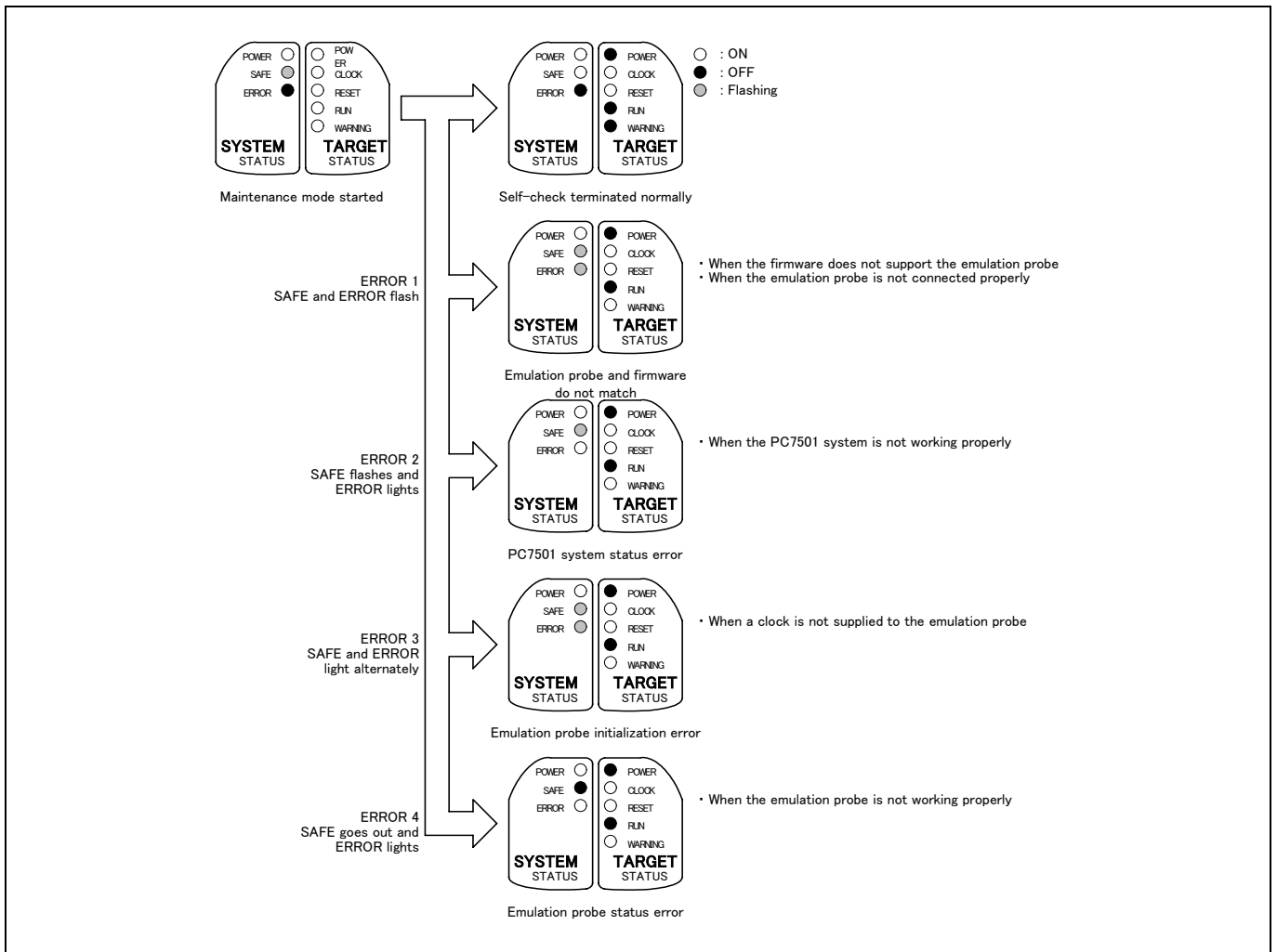
Figure 2.6 Self-check procedure
